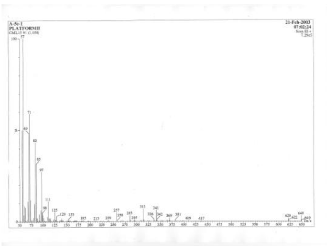
圖 7 : Mass spectrum of compound III
