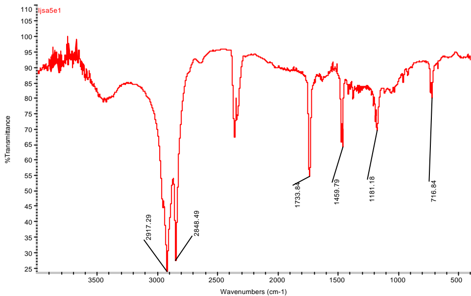
圖 6 : IR spectrum of compound III
